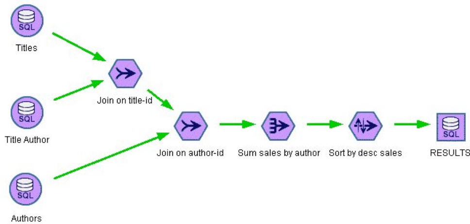
Figure 4: Entire stream executed in database
